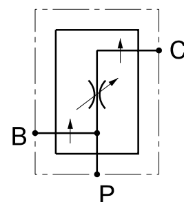
Schema idraulico Hydraulic scheme
